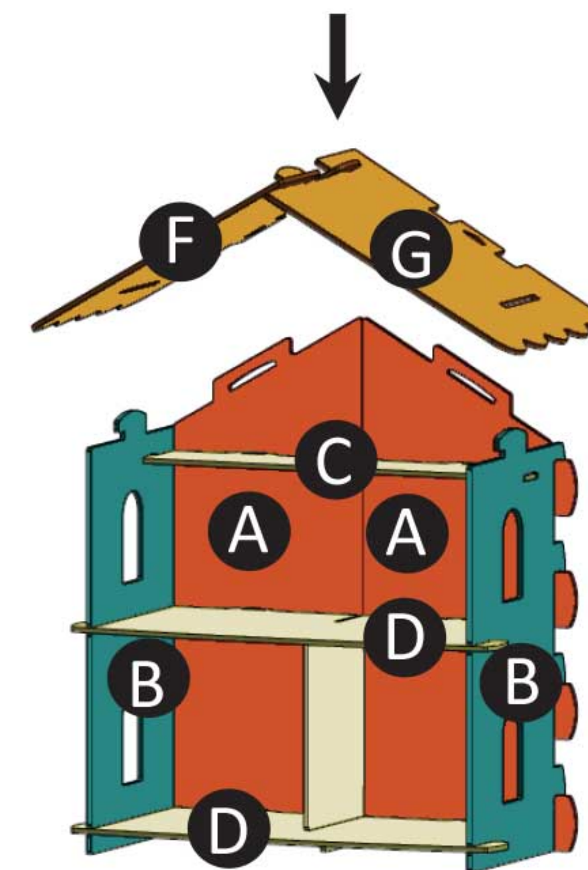
7. Fit roof panel slots (Fig. F and G) onto side wall tabs (Fig. B) at the same time. Then, slide roof tabs into back panels (Fig. A) at the same time. Push dowel rods through holes in the tabs of the roof (Fig. F and G), and two floor panels (Fig. D) along the back side of the house.
