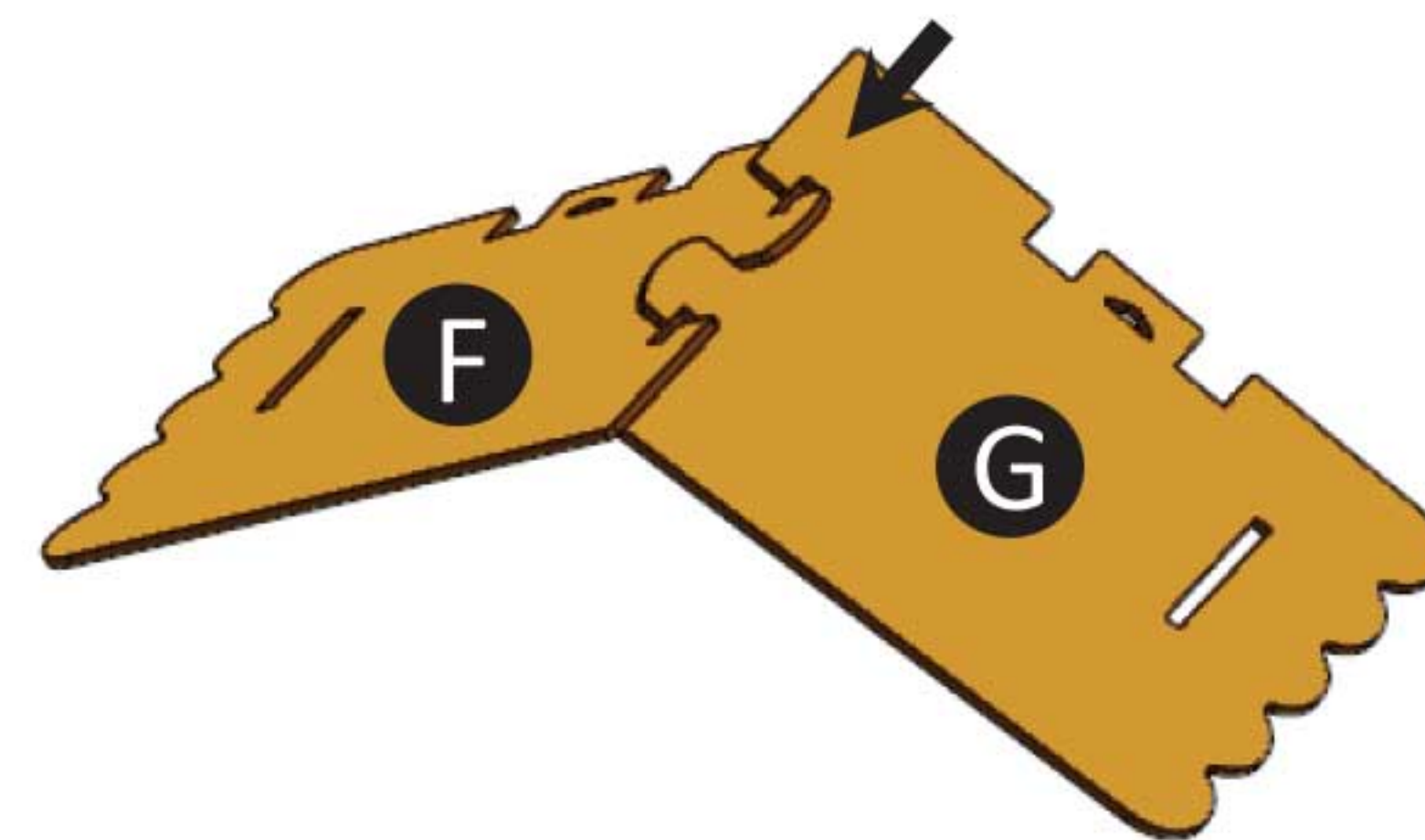
6. Interlock two roof panels (Fig. F and G) apart from the structure.
